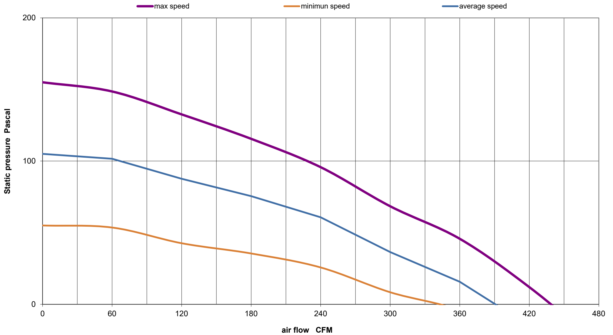
FRC 140 CL model- static pressure room air - (evaporator in summer mode)
